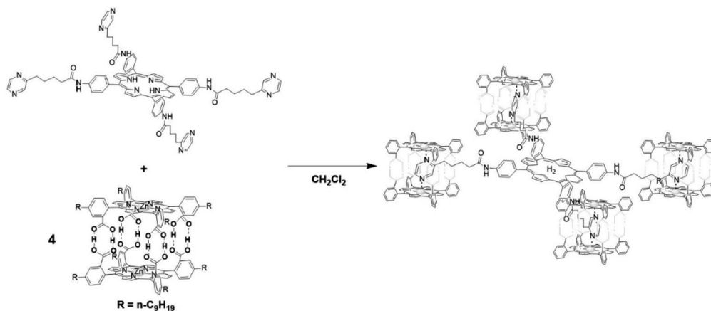
Fig. 4 A porphyrin acceptor functionalized with ditopic pyrazine units (top) that act as guests to the donor Zn-porphyrin cage assembled with hydrogen bonds. A 8 : 1 donor : acceptor ratio is achieved here. Some atoms in the antenna system are omitted for clarity.
