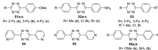
Fig. 2 Chemical structure of tetrazine derivatives 51–56 .
