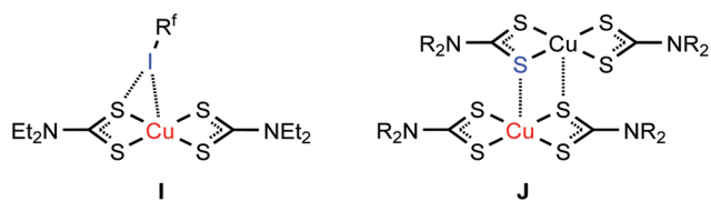
Fig. 6 C–I...(S–Cu) contact in the structure of 1:2FIB (I) and the dimerization of [\text{Cu}^{\text{II}}(\text{S}_2\text{CNR}_2)_2] (J) via Cu II ...S semicoordination.
