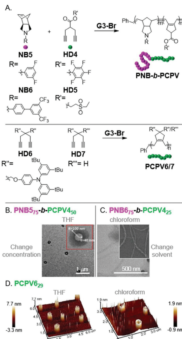
Fig. 7 (A) Synthesis of PNB- b -PCPV and PCPV6/7. (B) TEM (on a carbon-coated copper grid) image of PNB5 75 - b -PCPV4 50 -based vesicles formed by changing solvent concentration. Adapted from ref. 50 with permission from the Royal Society of Chemistry, copyright 2015. (C) TEM (on a carbon-coated copper grid) image of PNB6 75 - b -PCPV4 25 -based nanotubes formed by changing the dispersion solvent. Adapted from ref. 51 with permission from the Royal Society of Chemistry, copyright 2017. (D) 3D AFM (on mica) images of cylindrical nano-objects from PCPV6. Adapted from ref. 53 with permission from American Chemical Society, copyright 2015.
