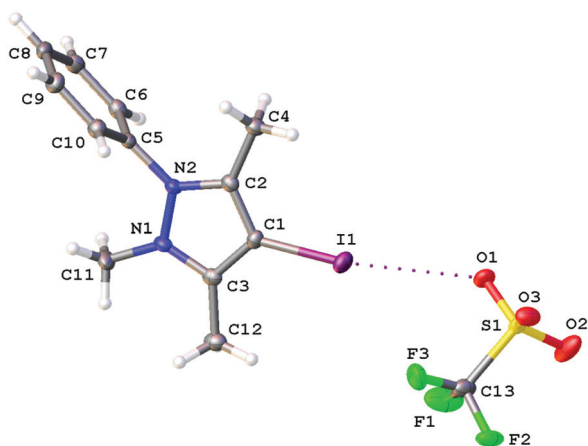
Fig. 3 The molecular structure of [5]OTf determined by X-ray diffraction.
