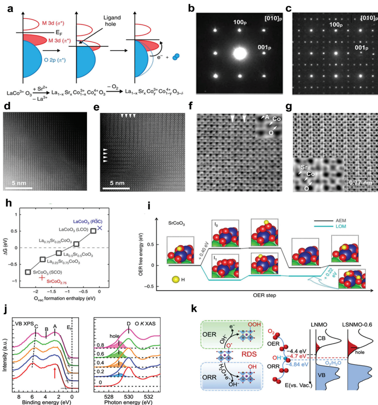
Fig. 3 (a) Schematic representation of the relationship between the oxygen vacancy concentration and Co–O bond covalency through Sr 2+ doping. SAED patterns of (b) \text{La}_{0.8}\text{Sr}_{0.2}\text{CoO}_3 and (c) \text{SrCoO}_3 . HAADF-STEM images of (d) \text{La}_{0.8}\text{Sr}_{0.2}\text{CoO}_3 and (e) \text{SrCoO}_3 . ABF-STEM imaging of oxygen vacancy ordering in (f) \text{La}_{0.2}\text{Sr}_{0.8}\text{CoO}_3 and (g) \text{SrCoO}_3 . (h) \Delta G (free energy difference between the LOM and AEM) versus the oxygen vacancy formation energy in perovskite oxides with different Sr 2+ concentrations. (i) The OER free energy changes of the LOM and AEM on \text{SrCoO}_3 . Reproduced with permission from ref. 67. Copyright 2014, Nature Publishing Group. (j) X-ray photoemission spectroscopy valence band and O K-edge XAS spectra of LSNMO with different Sr 2+ concentration. (k) Left panel: rate-determining step of the OER and the ORR. Right panel: schematics diagram for the electronic structure near the Sr Fermi level. Reproduced with permission from ref. 70. Copyright 2021, American Chemical Society.
