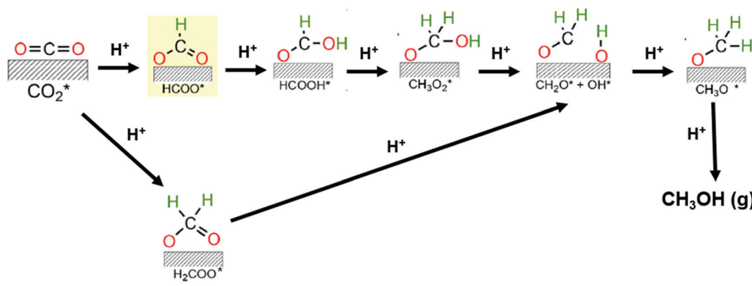
Fig. 2 Proposed reaction mechanisms for the CO 2 hydrogenation toward methanol. Adapted from ref. 45 and 46.
