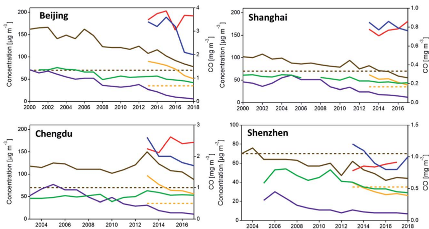
Fig. 7 Air quality trends (annual average) for Beijing, Shanghai, Shenzhen and Chengdu. Red, O 3 ; blue, CO; green, NO 2 ; purple, SO 2 ; brown, PM 10 (dotted brown line, PM 10 standard); yellow, PM 2.5 (dotted yellow line – PM 2.5 standard). Note O 3 level = annual average of daily 8 h mean concentration. Sources: China Statistics Bureau and Beijing Environmental Protection Bureau; China Statistics Bureau and Shanghai Environmental Protection Bureau; China Statistics Bureau and Shenzhen Environmental Protection Bureau; China Statistics Bureau and Chengdu Environmental Protection Bureau (data compiled by W. Wan 167 ).
