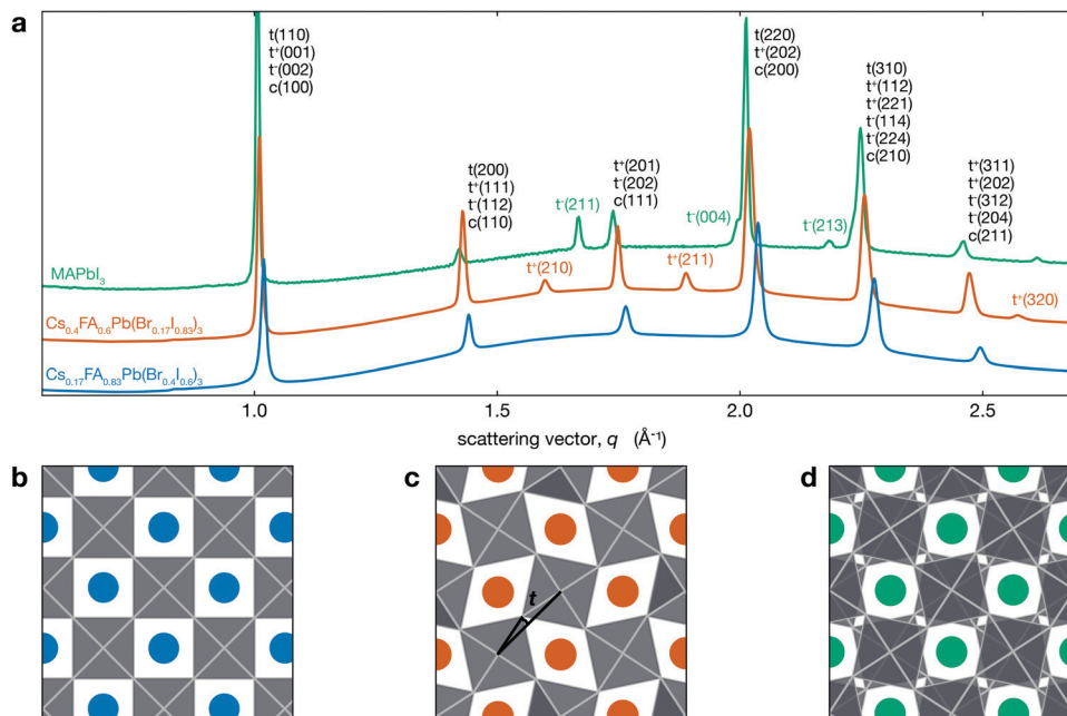
Fig. 1 (a) XRD patterns for different \text{Cs}_x\text{FA}_{1-x}\text{Pb}(\text{Br}_{x/1-x}\text{I}_{1-x/1-x})_3 compositions exhibiting both tetragonal \text{a}^0\text{a}^0\text{c}^+ (tetragonal peaks indexed with t^+ ) and cubic \text{a}^0\text{a}^0\text{a}^0 structures as well as the \text{a}^0\text{a}^0\text{c}^- (tetragonal peaks indexed with t^- ) phase of \text{MAPbI}_3 ( \text{MAPbI}_3 data from Schelhas et al. 50 ). The y-axis is linear in intensity (arbitrary units not shown) with an offset between the three patterns. Views of (b) \text{a}^0\text{a}^0\text{a}^0 , (c) \text{a}^0\text{a}^0\text{c}^+ , and (d) \text{a}^0\text{a}^0\text{c}^- structures looking down the c -axis. Blue, orange and green spheres represent the A-site cation, and the \text{PBX}_6 octahedra are shown in grey. The tilt angle t we consider here is the angle between the black lines in (c).
