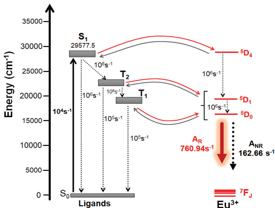
Fig. 6 Schematic energy-level diagram showing the most important ET channels for [Eu(btfa) 3 1c]. Please see Table 5 for the corresponding values of ET rates.
