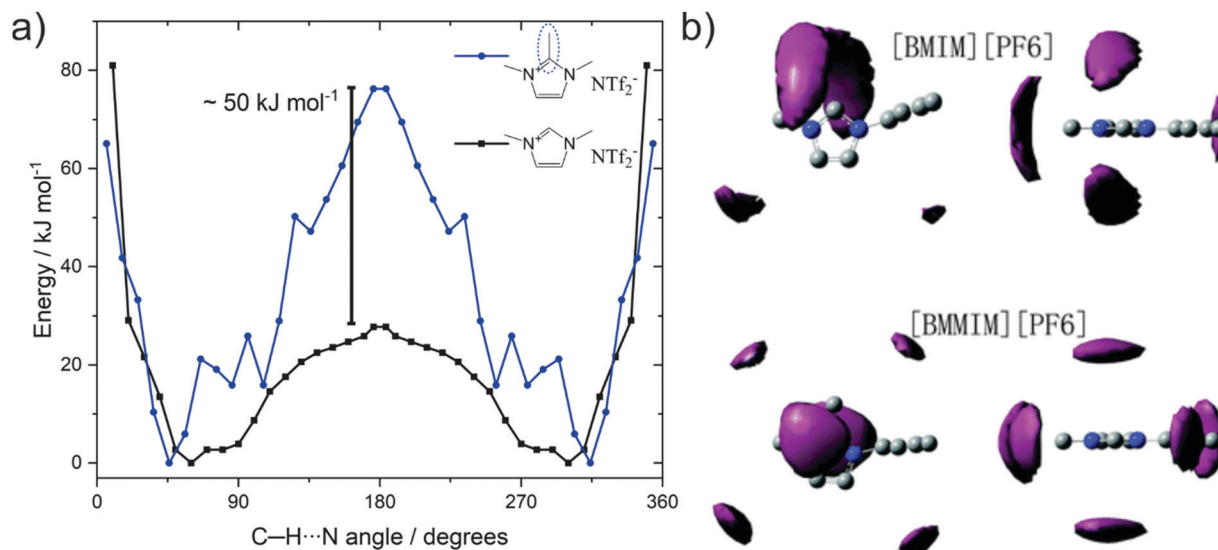
Fig. 20 (a) Energy as a function of the angle between C2 carbon, acidic hydrogen, and imide-N of the [NTf 2 ]. 255 (b) Spatial distribution function of [PF 6 ] - around [C 4 C 1 im] + (top) and [C 2 -methylated C 4 C 1 im] + (bottom). Reproduced from ref. 257 with permission from the PCCP Owner Societies.
