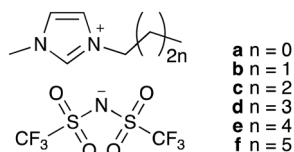
Fig. 1 The methylimidazolium-based ionic liquids 4a–f that were used herein.
