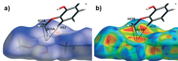
Fig. 7 The d_{\text{norm}} (a) and shape index (b) Hirshfeld surfaces for 1 , highlighting the inter-chain C–H \cdots\pi interactions: C12(H12)\cdots [C9-C14]_{\text{centroid}} = 3.10 Å; C15(H15A)\cdots [C9-C14]_{\text{centroid}} = 3.53 Å and C12(H15B)\cdots [C9-C14]_{\text{centroid}} = 3.48 Å (these are distances taken from the crystal structure data).
