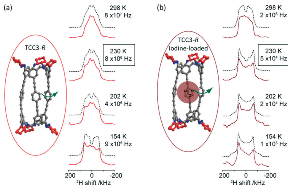
Fig. 3 (a) TCC3-R structure (red) and variable temperature ^2\text{H} static solid echo NMR spectra of [\text{D}_{12}] TCC3-R. (b) Iodine-loaded TCC3-R structure (burgundy) and variable temperature ^2\text{H} static solid echo NMR spectra of iodine loaded [\text{D}_{12}] TCC3-R. Corresponding simulated spectra (black dashed lines) and rotational rates obtained from numerical simulations of the NMR lineshape obtained at various temperatures are also given. In the crystal structures, the cyclohexane groups are represented in red; other C, grey; N, blue; H/D omitted for clarity. Ref. 48 is an open access article distributed under the terms of the Creative Commons CC BY license.
