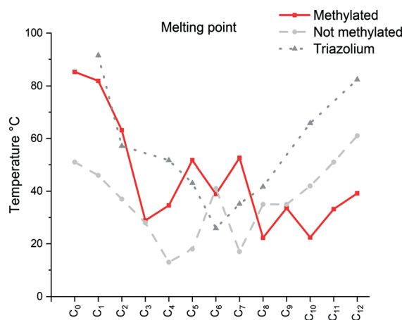
Fig. 1 Comparison of the melting point ( \text{Cr} \rightarrow \text{Sm}/L_{\text{iso}} ) of the [C_{12}C_n\text{Im}][\text{Br}] (methylated), [C_{12}C_n\text{Im}][\text{Br}] (not methylated) 42 and [C_{12}C_n\text{Tr}][\text{Br}] (1,2,3-triazolium). 46
