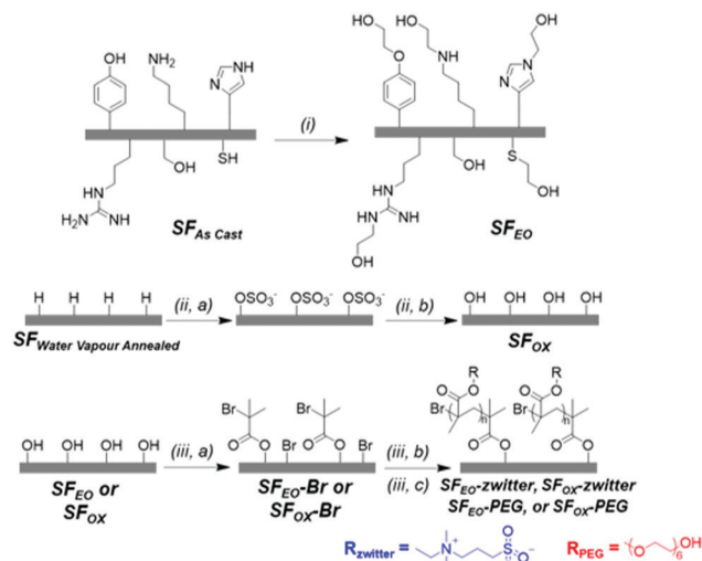
Scheme 2 (i) Ethylene oxide treatment of unmodified silk fibroin (SF) films to result in \text{SF}_{\text{EO}} ; (ii, a) oxidation of unmodified SF films using ammonium persulfate [aqueous 15% w/v APS, 5 min, 25 °C] and (ii, b) hydrolysis of organosulfate groups to hydroxyl groups [ \text{dH}_2\text{O} , 10 min, 25 °C] to result in \text{SF}_{\text{OX}} ; (iii, a) initiator attachment to hydroxylated SF films [ \text{NEt}_3 , BIBB, chloroform, 4 h, 40 °C], (iii, b) ATRP of zwitterionic monomer [ \text{CuBr/Bipy} , DMAPS, methanol/water, 12 h, 25 °C] and (iii, c) ATRP of PEGMA monomer [ \text{CuBr/Bipy} , PEGMA, methanol/water, 12 h, 25 °C]. Reaction (ii) has the potential to modify the amide backbone as well as numerous amino acid residues, therefore this scheme is not drawn to show the individual reactive sites that are modified.
