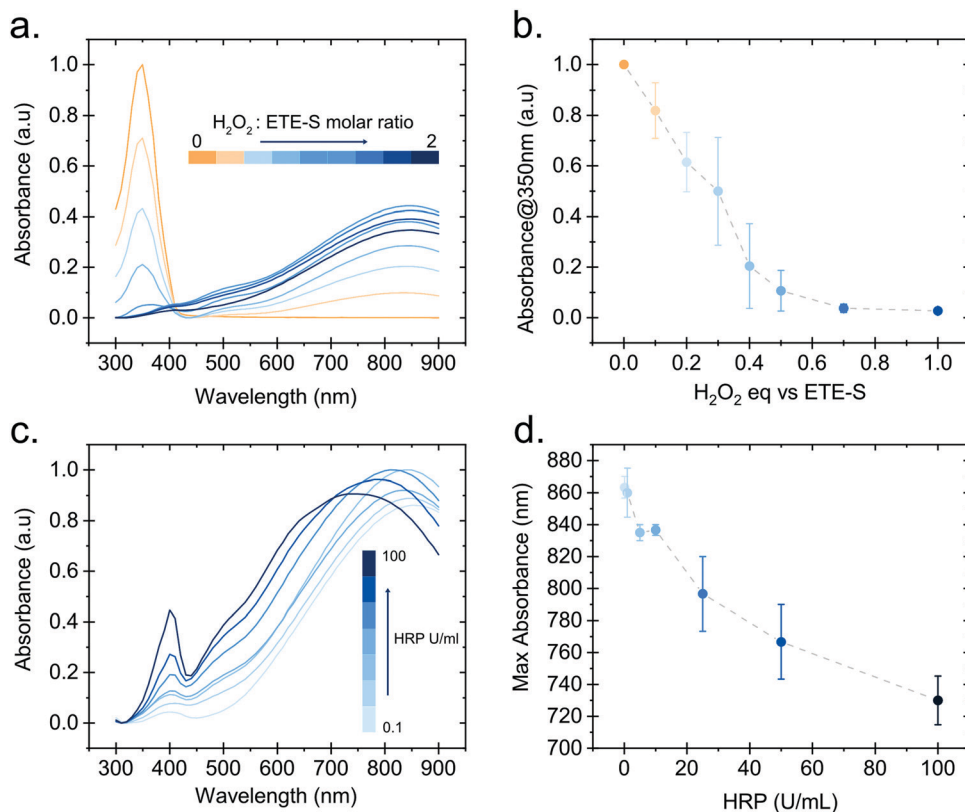
Fig. 3 Effect of \text{H}_2\text{O}_2 and HRP concentration on the ETE-S in vitro polymerization. (a) Absorption spectra of p(ETE-S) formed in vitro with 5 U ml -1 HRP and various molar equivalents of \text{H}_2\text{O}_2 to ETE-S. (b) Absorbance at 350 nm for the spectra shown in (a) as a function of the molar equivalents of \text{H}_2\text{O}_2 to ETE-S. (c) Absorption spectra of p(ETE-S) formed in vitro for various HRP concentrations. (d) Wavelength corresponding to the highest absorbance value in (c) as a function of the HRP concentration. For (b) and (d) n = 3 .
