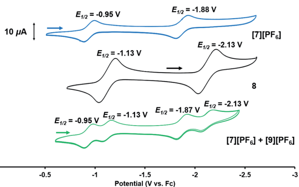
Fig. 7 Cyclic voltammograms (in 0.3 M [ 7 ]Bu _4 N][PF _6 ] in THF; scan rate: 100 mV s ^{-1} ) of compounds [ 7 ][PF _6 ] (blue), 8 (black), and a mixture of [ 7 ][PF _6 ] and [ 9 ][PF _6 ] obtained from the reaction of 8 with FcPF _6 (green).
