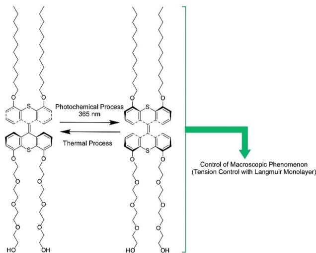
Fig. 12 The bidirectional control of the surface tension of a macroscopic liquid surface through the photo-switching of a photoactive amphiphile with a bis(thiaphenylidene) unit.
