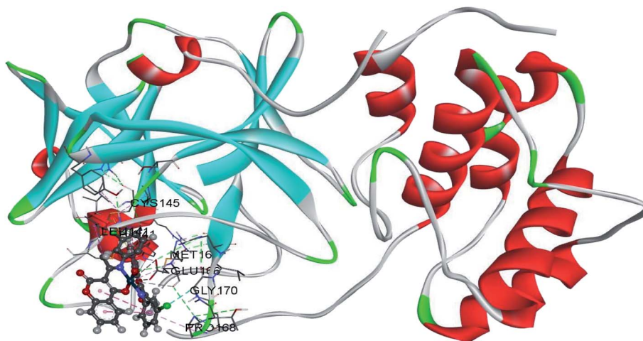
Fig. 5 The docking interactions of the most stable conformation of ligand (Pd(II) complex) with M^{\text{PrO}} of SARS-CoV-2.
