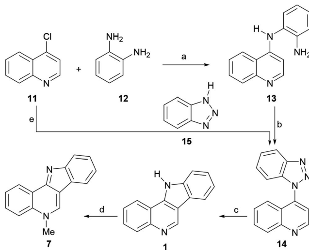
Scheme 1 Reagents and conditions: (a) 140 °C, 20–30 mm Hg, 10–20 min (76%); (b) NaNO 2 , 1 N HCl, H 2 O, 5 °C (70%); (c) H 3 PO 4 , heat (77%); (d) MeI, PhNO 2 , 2 h, 100 °C (72%); (e) (1) 15 , MW (160 W); (2) pyrophosphoric acid, 160 W, 4–6 min (60% overall).
