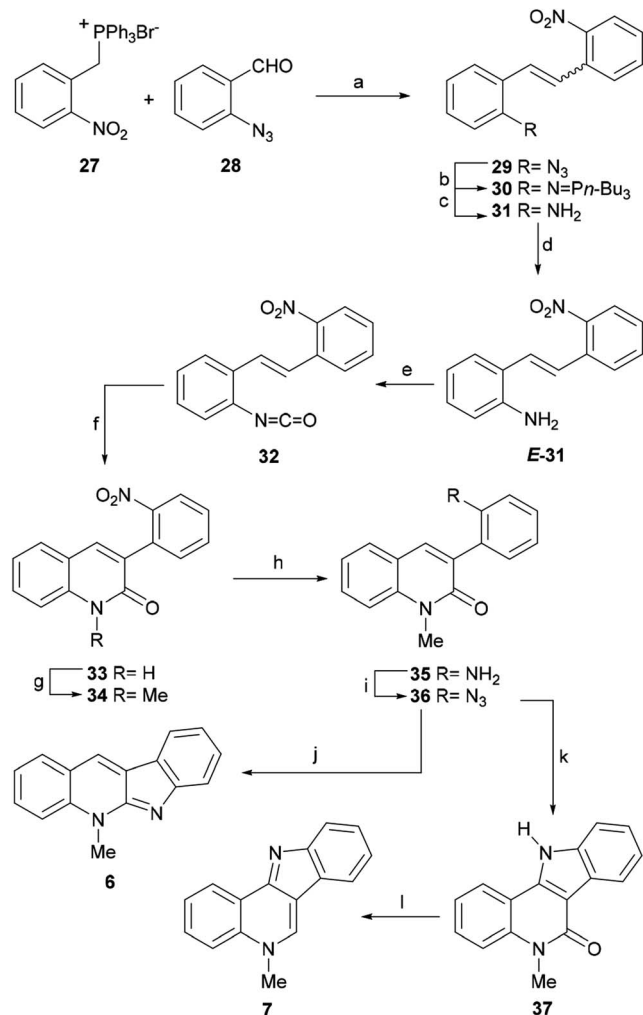
Scheme 7 Reagents and conditions: (a) \text{K}_2\text{CO}_3 , dibenzo-18-crown-6, \text{CH}_2\text{Cl}_2 , rt (85%, Z/E = 4:1 ); (b) n\text{-Bu}_3\text{P} , \text{CH}_2\text{Cl}_2 , rt; (c) \text{THF-H}_2\text{O} , rt (84%, Z/E = 7:1 ); (d) \text{PhSH} , AIBN, \text{PhH} , reflux (92%); (e) triphosgene, \text{CH}_2\text{Cl}_2 , \text{Et}_3\text{N} , 0^\circ\text{C} \rightarrow \text{rt} , 1 h; (f) \text{PhNO}_2 , MW, 150^\circ\text{C} , 12 min (80% overall); (g) \text{CH}_3\text{I} , DMF, 60^\circ\text{C} (82%); (h) \text{H}_2 , Pd/C, EtOH, rt (91%); (i) (1) \text{NaNO}_2 , \text{H}_2\text{SO}_4 ; (2) \text{NaN}_3 , \text{H}_2\text{O} (85%); (j) (1) \text{Me}_3\text{P} , \text{PhNO}_2 , rt, 45 min; (2) MW, 180^\circ\text{C} , 30 min (40% overall); (k) o\text{-xylene} , 150^\circ\text{C} (82%); (l) Red-Al, \text{PhMe} , reflux, 32 h (90%).
