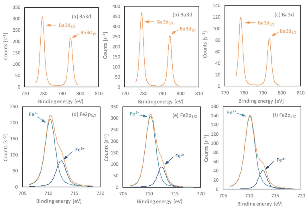
Fig. 3 XPS signals of Ba and Fe elements, obtained for pure \text{BaFe}_{12}\text{O}_{19} samples \text{BaM}_{10\_1} (a and d), \text{BaM}_{12\_2} (b and e) and \text{BaM}_{12\_3} (c and f).
