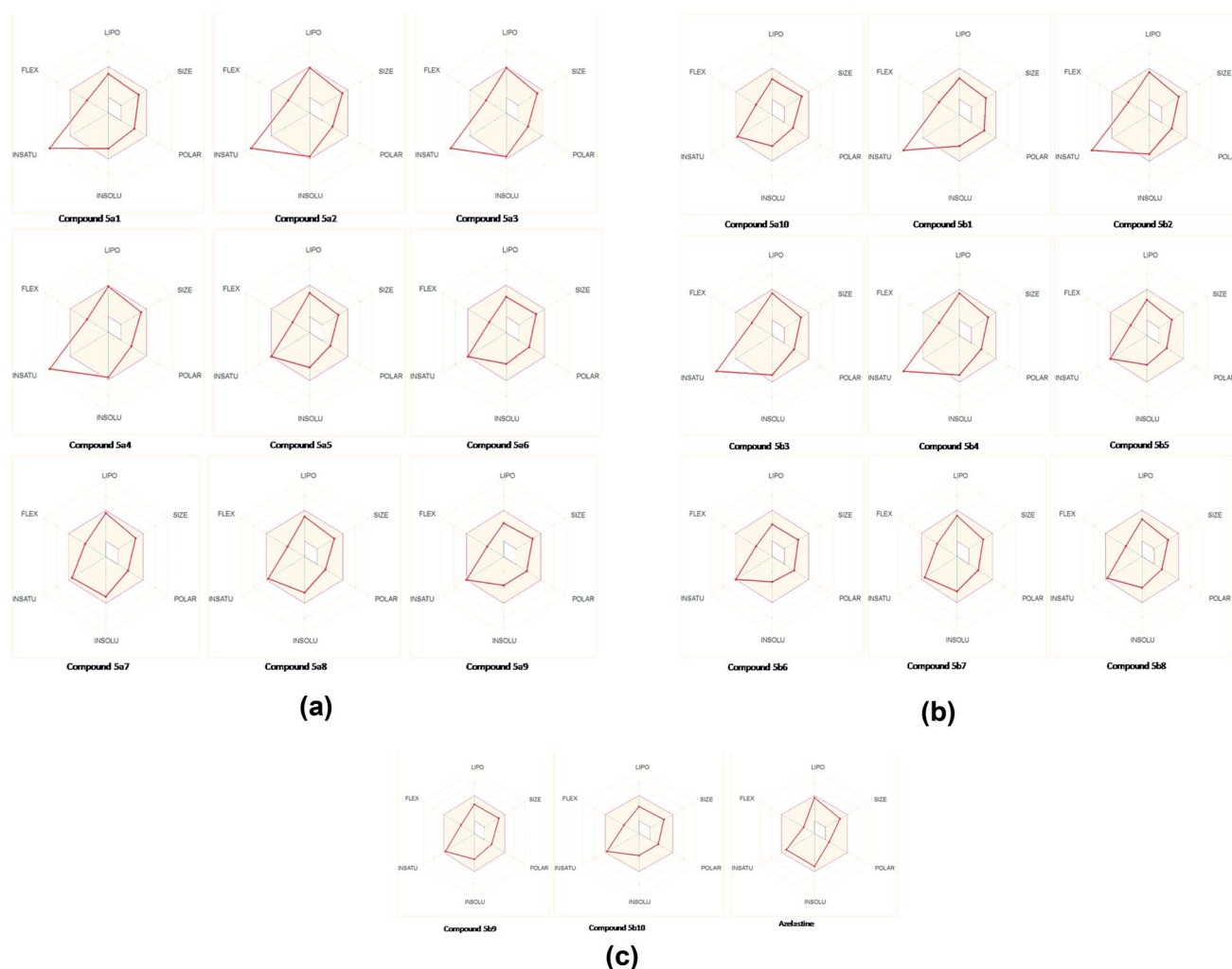
Fig. 5 (a) Bioavailability radar graph of 1,8-naphthyridine derivatives 5a1–5a9 (pink area reflects the allowed values of drug-likeness properties of the molecule). (b) Bioavailability radar graph of 1,8-naphthyridine derivatives 5b10–5b8 (pink area reflects the allowed values of drug-likeness properties of the molecule). (c) Bioavailability radar graph of 1,8-naphthyridine derivatives 5b9–5b10 (pink area reflects the allowed values of drug-likeness properties of the molecule).
