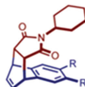
Fig. 34 Pair-selective encapsulation followed by Diels–Alder reaction and yields of regioselective syn -1,4-products in cage I . Reproduced with permission from ref. 123. Copyright 2006, American Association for the Advancement of Science.
