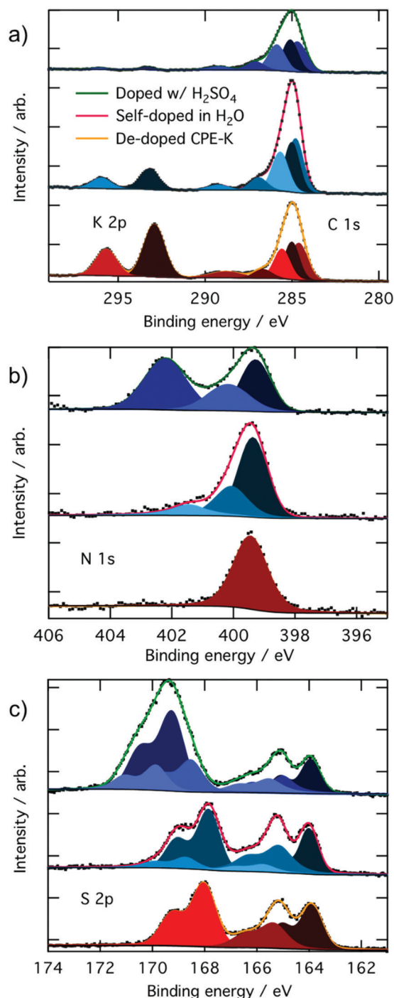
Fig. 2 High resolution XPS spectra of (a) C 1s and K 2p 3/2 , (b) N 1s, and (c) S 2p 3/2 and their Voigt fitting profiles of CPE-K w/H 2 SO 4 added, self-doped CPE-K, and de-doped CPE-K on ITO with a film thickness of 20 nm. Black dots are experimental data and the colored lines are overall fits obtained with a peak-fitting routine.
