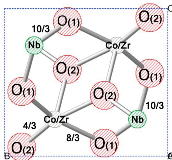
Fig. 38 The coordination number and charge distribution of ions in \text{AZrNb}_2\text{O}_8 ceramics (here A = Co ions) (reprinted with permission from ref. 218. Copyright 2016 Elsevier).
