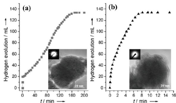
Fig. 1 Hydrogen generation by hydrolysis of aqueous AB (0.16 m, 10 mL) in the presence of (a) the pre-synthesized and (b) in situ synthesized Fe catalysts (Fe/AB = 0.12) at room temperature under argon. The inset shows the corresponding TEM images and SAED patterns of the as-synthesized catalysts. Reprinted with permission from ref. 155. Copyright (2008) Wiley-VCH.
