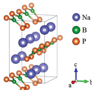
Fig. 28 Crystallographic structure of Na 2 BP 2 .
