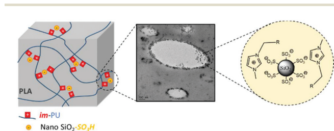
Fig. 19 Design of ultra-tough PLA-based ionic nanocomposites, based on polymer/particle ionic interactions with impact of a modifier-like morphology. Adapted from ref. 155. Copyright 2020 with permission from Elsevier.
