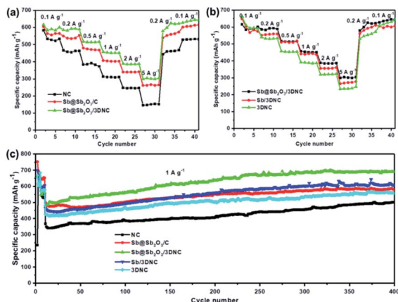
Fig. 6 (a and b) Rate capability and (c) cycling performance of the NC, Sb@Sb 2 O 3 /C, Sb@Sb 2 O 3 /3DNC, Sb/3DNC, and 3DNC.
