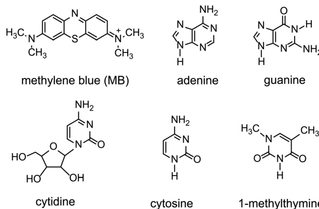
Scheme 2 Chemical structures of cationic and neutral molecules added into G4·M + (M + = K + , Na) borate gels. Cytidine is used as an external standard to quantify incorporation of adenine into G4·K + borate gels.
