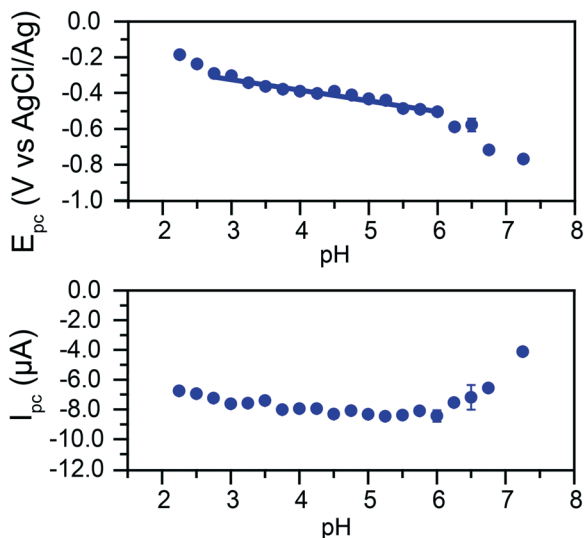
Fig. 5 Top: Cathodic peak potentials, with standard deviations, as a function of pH. The linear fit in the 2.75 to 6 pH range has a slope of 59.6 mV \text{pH}^{-1} (adj. R^2 = 0.948 ). Bottom: Cathodic faradic peak currents, with standard deviations, as a function of pH. Data collected in a 0.1 M citric acid buffer with 1 M KCl as supporting electrolyte and in the presence of 200 \mu\text{M} of potassium chromate.
