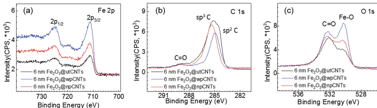
Fig. 5 (a) High-resolution Fe 2p spectra; (b) C 1s spectra and (c) O 1s spectra of 6 nm \text{Fe}_2\text{O}_3 @CNTs.
