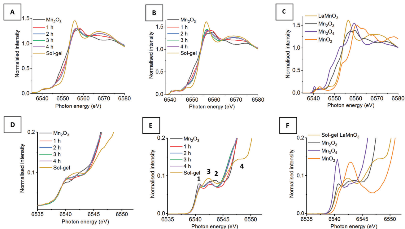
Fig. 1 (A) XAS Mn K-edge XANES compared to (B) HERFD-XANES of time-slices during the mechanochemical synthesis of \text{LaMnO}_3 compared to (C) reference Mn(II), (III), (IV) oxides and sol-gel synthesised \text{LaMnO}_3 with (D–F) their respective highlighted pre-edge region.
