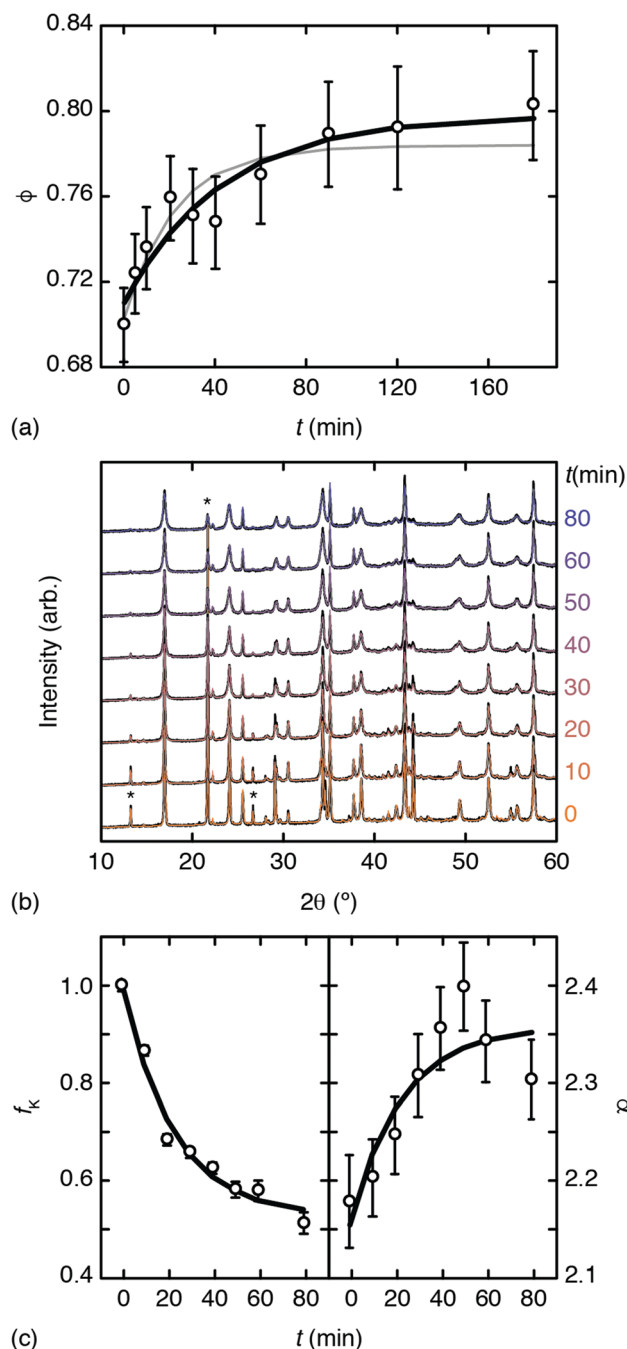
Fig. 2 Evidence for mechanochemical vacancy filling in Mn[Co(CN)_6]_{2/3} . (a) Variation in Co/Mn ratio with milling time as determined using ICP. The bold line shows the fit to data obtained using eqn (1); the fine grey line is the corresponding fit when all data sets are included. (b) PXRD traces (black lines) and fits (coloured lines) for milled samples; successive curves are shifted vertically by a constant amount. Three reflections associated with K_3[Co(CN)_6] are marked with an asterisk. (c) Phase fractions and intensity ratios extracted from (b) as discussed in the text. The bold lines show the fit-to-data using eqn (1).
