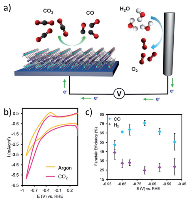
Fig. 9 (a) Schematic showing a thin film cobalt-porphyrin MOF, \text{Al}_2(\text{OH})_2\text{TCPP-Co} , performing CO 2 reduction. (b) An increase in current is observed in the cyclic voltammogram when the MOF is subjected to a CO 2 environment. (c) Selectivity for generation of CO and H 2 was tested over the potential range -0.5 to -0.9 \text{ V} vs. RHE with a reported peak faradaic efficiency for CO of 76%. Adapted with permission. 158 Copyright 2015 American Chemical Society.
