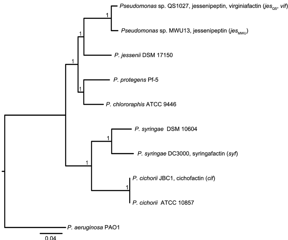
Fig. 6 Top: Molecular phylogeny of the lipopeptide-producing Pseudomonas species based on multilocus sequence typing (MLST) of 16S rRNA genes and five housekeeping genes ( gyrB , nucD , IleS , ppsA , rpoB ). The tree was inferred by Maximum Likelihood estimation using a concatenated alignment as input. The P. aeruginosa PAO1 sequence was used as an outgroup to root the tree. The scale bar indicates substitutions per site.
