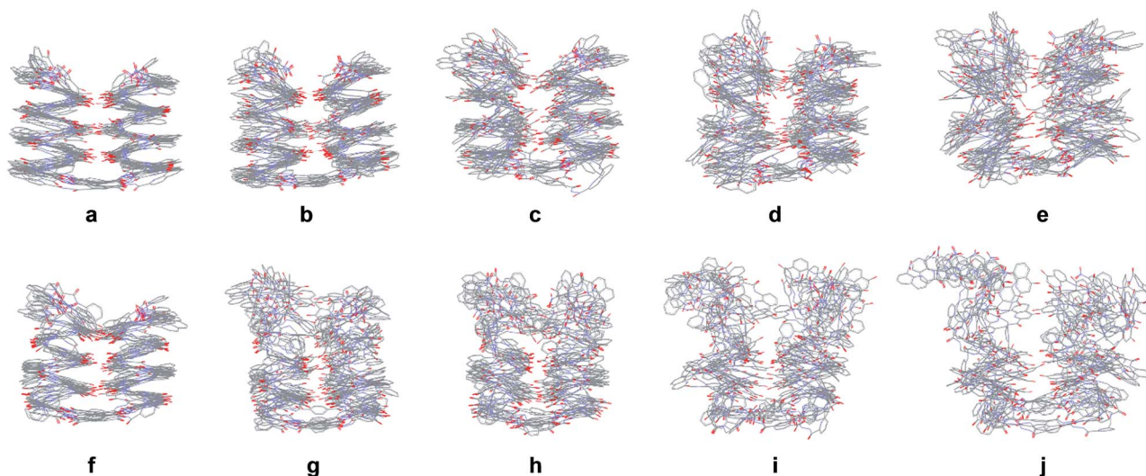
Fig. 8 Stochastic dynamic simulations of 5b in CHCl 3 over 1 ns at 300 K (a), 400 K (b), 500 K (c), 600 K (d) and 700 K (e). Stochastic dynamic simulations of 8b in CHCl 3 over 1 ns at 300 K (f), 400 K (g), 500 K (h), 600 K (i) and 700 K (j). In each case, ten structures sampled every 100 ps are overlaid for each temperature. Side chains of Q, P and T have been omitted for clarity.
