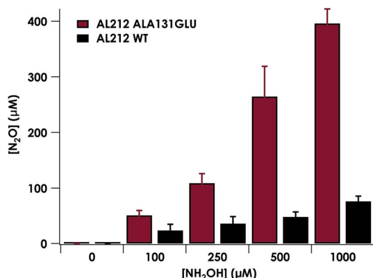
Fig. 6 Plot of N_2O production as a function of NH_2OH concentration by AL212 cyt P460 variants. Assay conditions were 5 µM cyt P460, 1 mM DCPIP, and NH_2OH concentrations ranging from 0–1 mM. Assays were carried out anaerobically in 200 mM HEPES, pH 8.0. Each data point is the average of at least three trials, with error bars representing one standard deviation.
