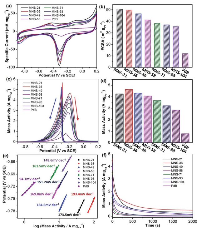
Fig. 5 Electrochemical EOR performance. (a) CV curves and (b) summarized ECSAs of trimetallic PdAgCu MNSSs with different sizes and commercial PdB obtained in 1.0 M KOH. (c) CV curves, (d) summarized mass activities, (e) Tafel plots, and (f) i - t curves of PdAgCu MNSSs and PdB collected in 1.0 M KOH and 1.0 M ethanol.
