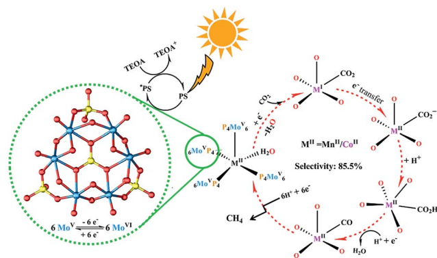
Fig. 4 Proposed mechanism for the photocatalytic reduction of \text{CO}_2 to \text{CH}_4 using NENU-605 and NENU-606 .
