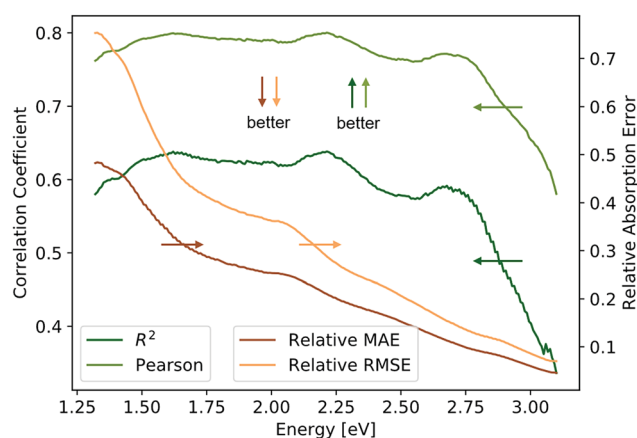
Fig. 4 Plot of the R^2 , Pearson, and relative MAE and RMSE along the energy axis for predicted spectra. The correlation coefficients are above 0.6 ( R^2 ) and 0.75 (Pearson) up until 2.75 eV. The lower MAE and RMSE above 2.75 eV are likely caused by less variation in the data due to consistently high optical absorption of ultraviolet light.
