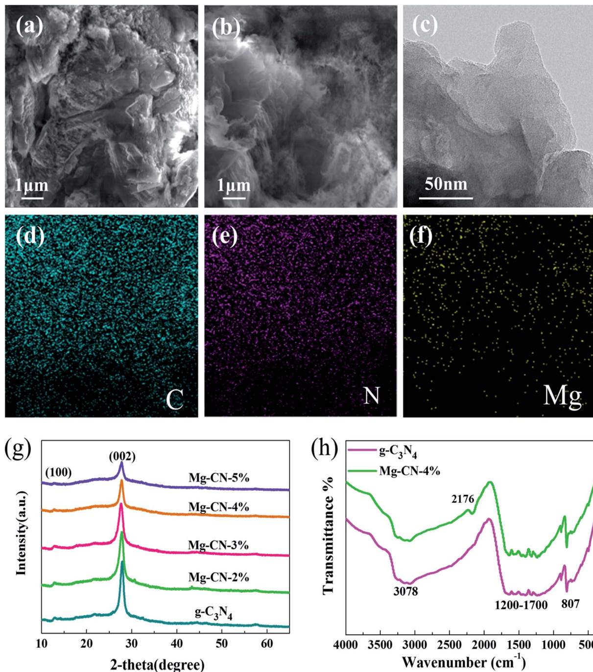
Fig. 1 SEM images of (a) g\text{-C}_3\text{N}_4 , (b) Mg-CN-4%; (c) TEM image of Mg-CN-4%; (d) elemental mapping images of C, (e) N, (f) Mg of Mg-CN-4%; (g) XRD spectra of samples; (h) FTIR spectra of g\text{-C}_3\text{N}_4 and Mg-CN-4%.
