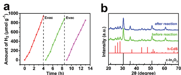
Fig. 8 (a) Photocatalytic stability of CdS/In 2 O 3 -2 towards visible-light hydrogen production; (b) XRD patterns of CdS/In 2 O 3 -2 before and after the photocatalytic cyclic test.
