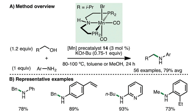
Scheme 22 Mn-Catalysed N -alkylation of arylamines (Beller).
