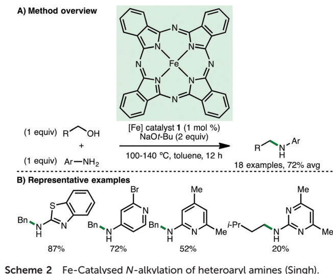
Scheme 2 Fe-Catalysed N -alkylation of heteroaryl amines (Singh).
