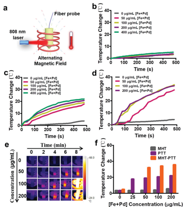
Fig. 2 Magnetic-photo dual-mode hyperthermia in aqueous solution. (a) Schematic diagram of the magnetic-photo dual-mode hyperthermia measurement system. Time dependent heating profiles of Fe 3 O 4 -Pd JNPs at various concentrations (b) under AMF (300 Oe; 350 kHz), (c) under 808 nm laser irradiation at a power density of 0.5 W cm -2 , and (d) under AMF plus 808 nm laser. (e) Thermal images acquired by the IR camera of Fe 3 O 4 -Pd JNPs at different concentrations under AMF plus 808 nm laser. (f) Average temperature increase recorded for Fe 3 O 4 -Pd JNPs under the three heating protocols.
