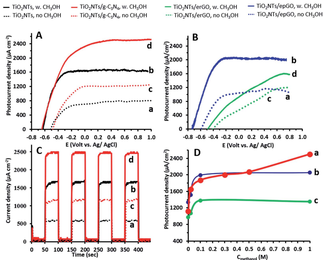
Fig. 2 (A) Linear sweep voltammograms ( 5 \text{ mV s}^{-1} ) in 0.1 \text{ M Na}_2\text{CO}_3 for TiO 2 NT (a and b) and TiO 2 NTs/g-C 3 N 4 (c and d) photoanodes in the absence and presence of 1 M methanol. (B) Linear sweep voltammograms ( 5 \text{ mV s}^{-1} ) in 0.1 \text{ M Na}_2\text{CO}_3 for TiO 2 NTs/epGO (a and b) and TiO 2 NTs/erGO (c and d) photoanodes in the absence and presence of 1 M methanol, respectively. (C) Current density versus time at a bias potential of +0.4 V vs. Ag/AgCl under chopped light irradiation for TiO 2 NT (a and b) and TiO 2 NTs/g-C 3 N 4 (c and d) photoanodes in the absence and presence of 1 M methanol, respectively. (D) Photocurrent density as a function of methanol concentration at a bias of +0.4 V for TiO 2 NTs/g-C 3 N 4 (a), TiO 2 NTs/epGO (b), and TiO 2 NTs/erGO (c) photoanodes.
