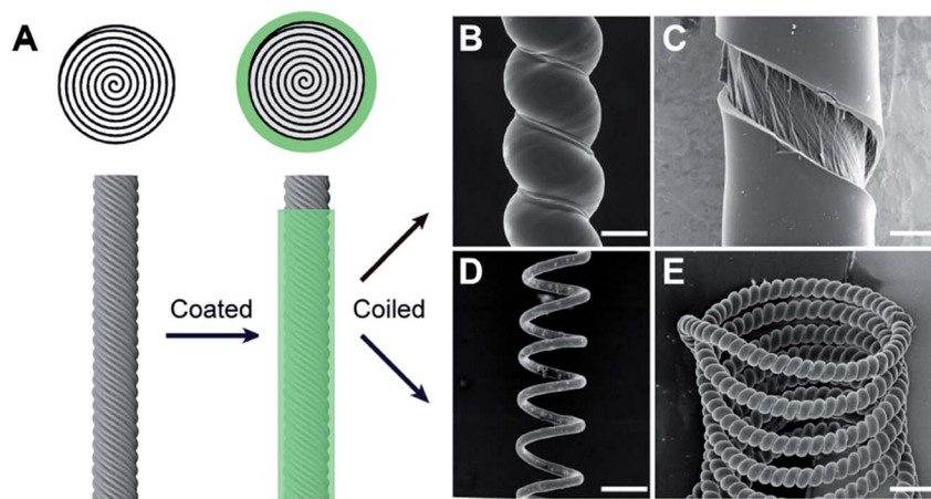
Fig. 24 Muscle fabrication and structures for torsional and tensile actuation. (A) Schematic lateral and cross-sectional views of a twisted CNT yarn and a SRAM, which was made by coating the twisted CNT yarn with a polymer sheath. SEM micrographs of PEO-SO 3 @CNT muscles showing (B) a SRAM made by self-coiling of a sheath-coated twisted yarn, (C) the surface of a twisted SRAM that was broken by untwisting in liquid N 2 , showing a distinct boundary between the sheath polymer and the CNT core, (D) a mandrel-coiled twisted SRAM, and (E) a SRAM that was self-coiled and then mandrel-coiled. The scale bars for (B)–(E) are 35, 15, 200, and 200 \mu m, respectively. This figure has been reproduced from ref. 9 with permission from AAAS.
