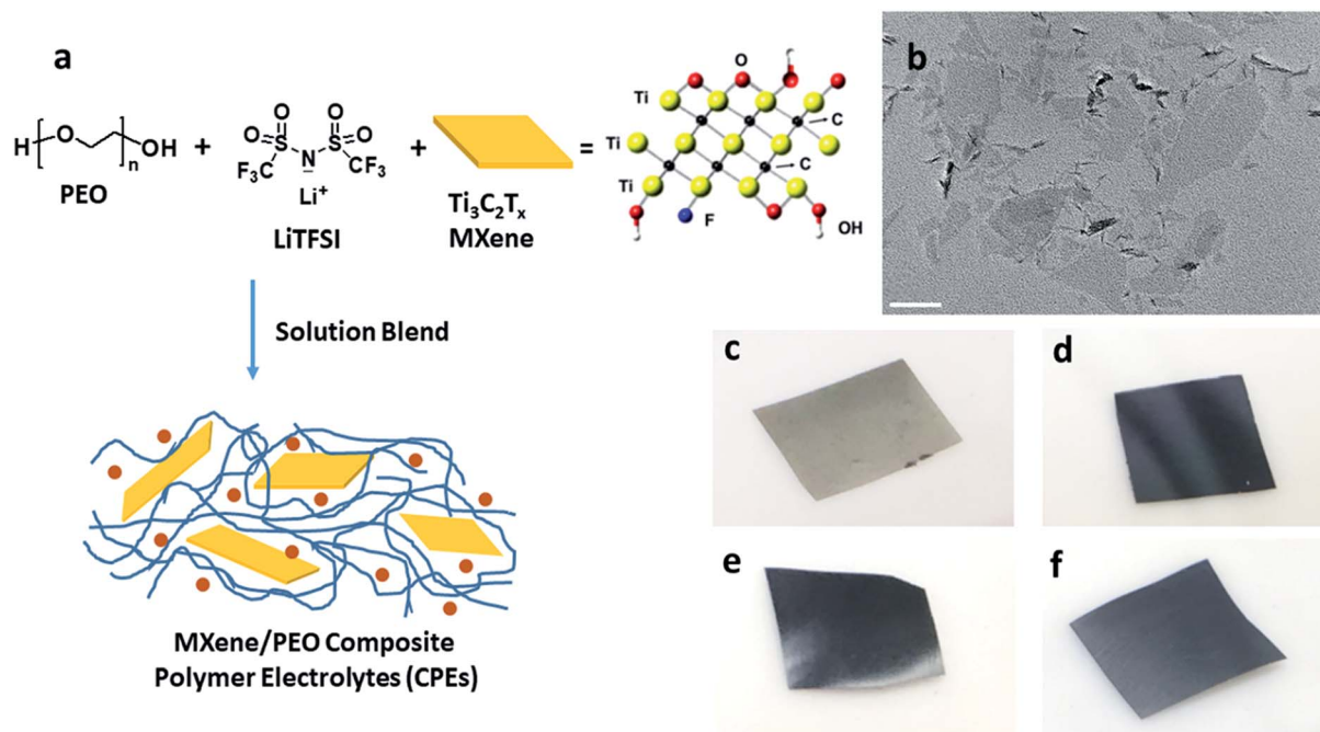
Fig. 1 Fabrication of MCPEs. (a) Preparation procedure of MCPEs. (b) TEM micrograph of the as-prepared few-layer MXene, scale bar is 100 nm. (c–f) Photographs of the MCPE membranes, (c) PEO_{20}-LiTFSI-MXene^{0.005} , (d) PEO_{20}-LiTFSI-MXene^{0.02} , (e) PEO_{20}-LiTFSI-MXene^{0.05} and (f) PEO_{20}-LiTFSI-MXene^{0.1} .
