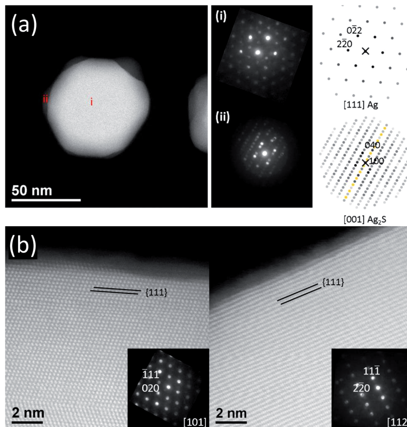
Fig. 3 (a) NBED diffraction patterns from a Ag 2 S/Ag particle after 8 min identify the phase as (i) Ag (space group 225, Fm \bar{3} m ) and (ii) Ag 2 S (space group 14, P2 1 / c ). Note in (i) forbidden reflections are present due to planar defects. The NBED patterns have been rotated to correspond to the orientation of the real space image and a nonlinear histogram adjustment was made to highlight the presence of weak features. Simulated diffraction patterns accompany the NBED patterns. (b) TEM Images of passivated surfaces. {111} surfaces after 24 h have only a thin Ag 2 S layer present. NBED patterns (inset) have been rotated to correspond to the orientation of the real space image and a nonlinear histogram adjustment was made to highlight the presence of weak features.
